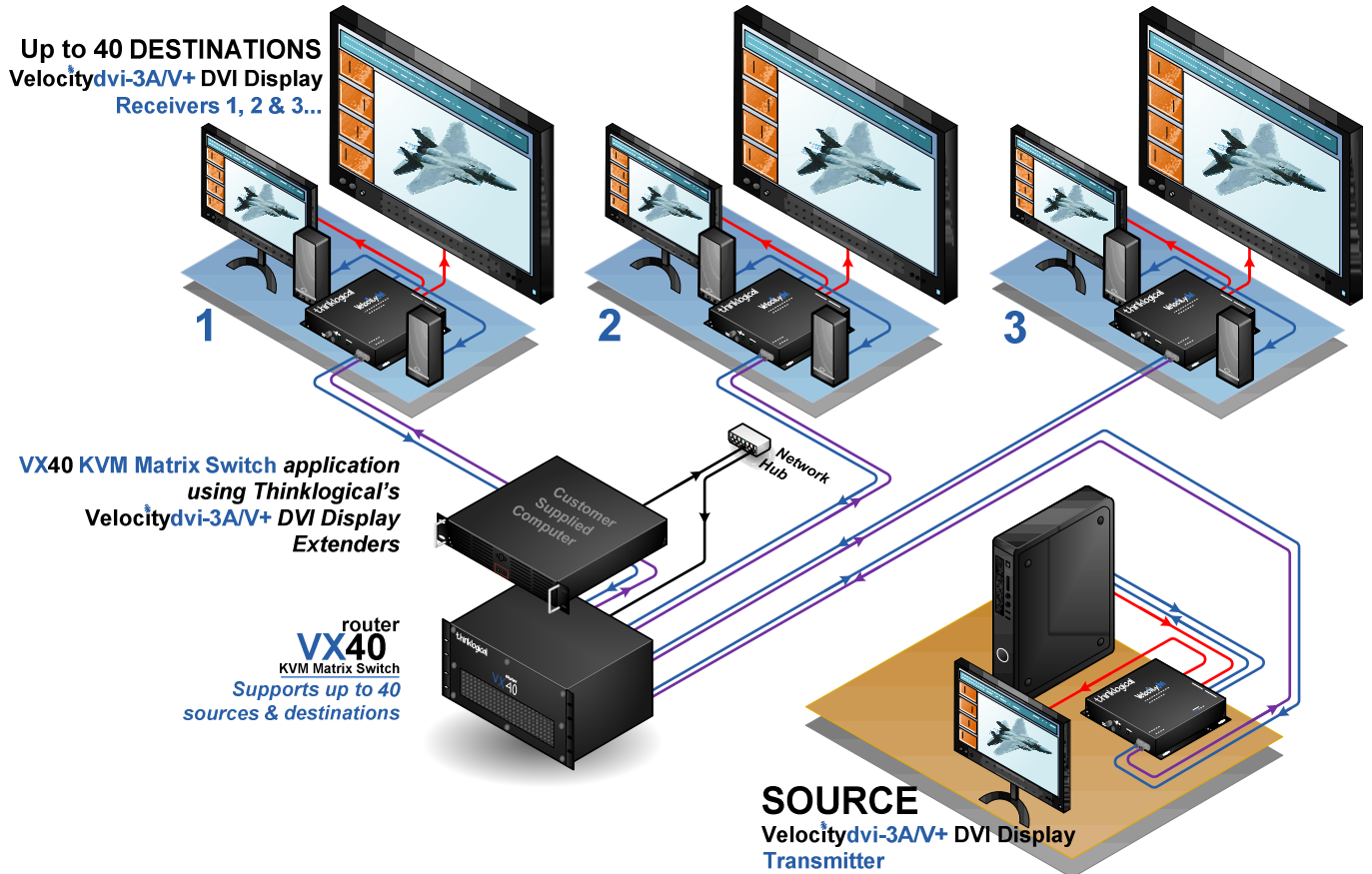
Typical VX40 Router Application using VelocityDVI-3AV+ Extenders
