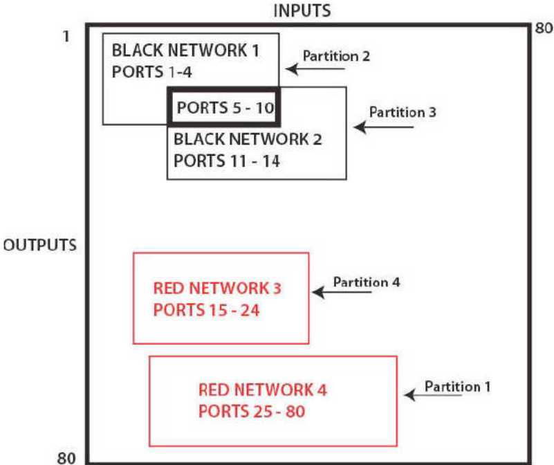
A VX80 with four partitions: Ports 5-10 are accessible to both partitions 2 and 3.
