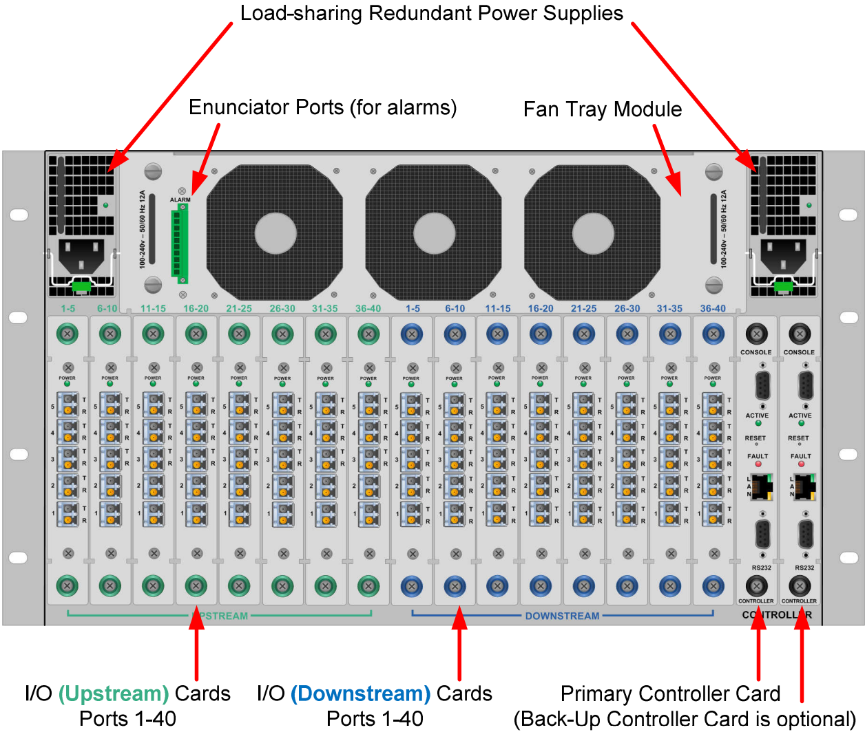
VX40 Router – Rear View
