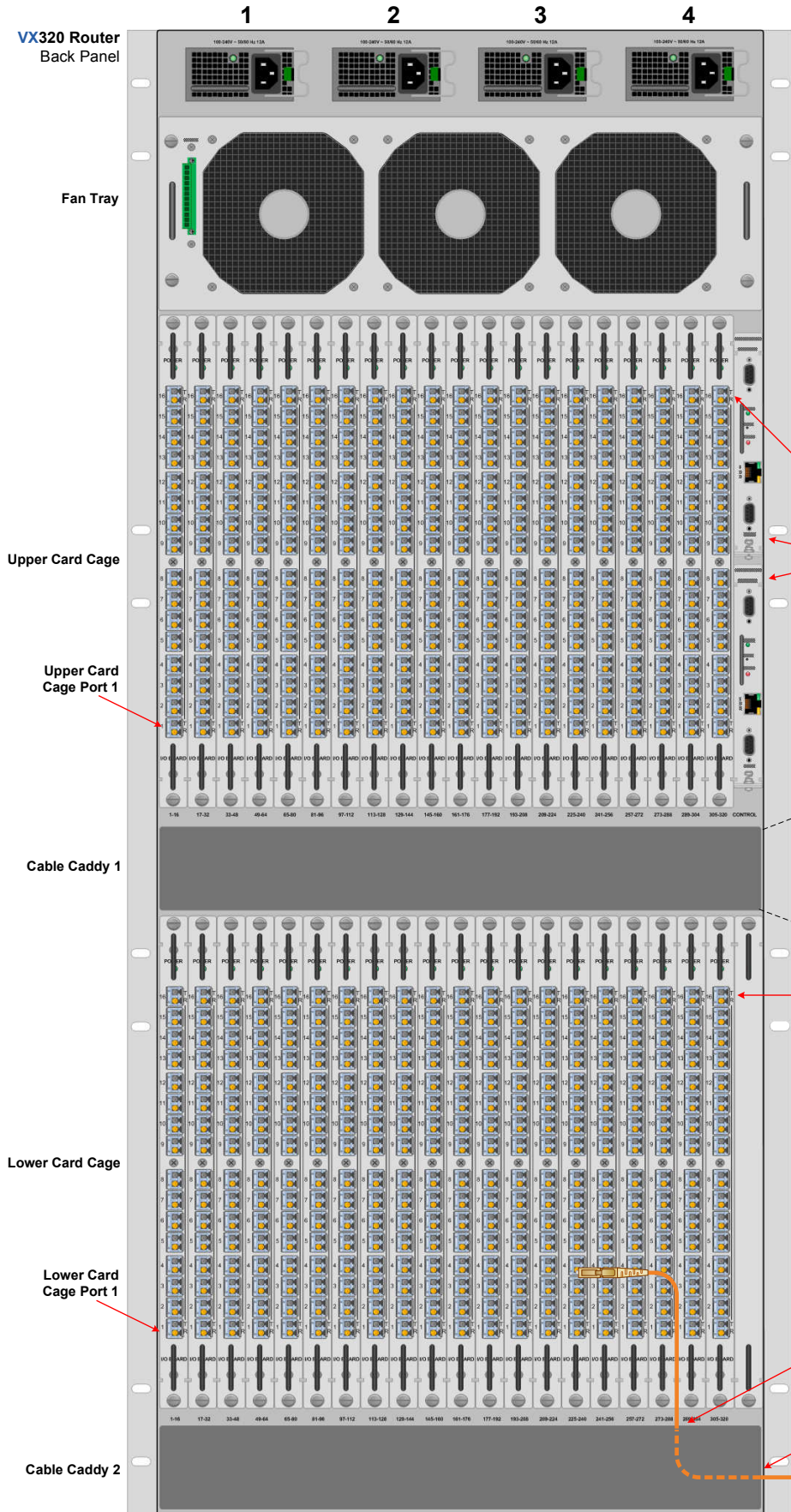
VX320 Router – Rear View
