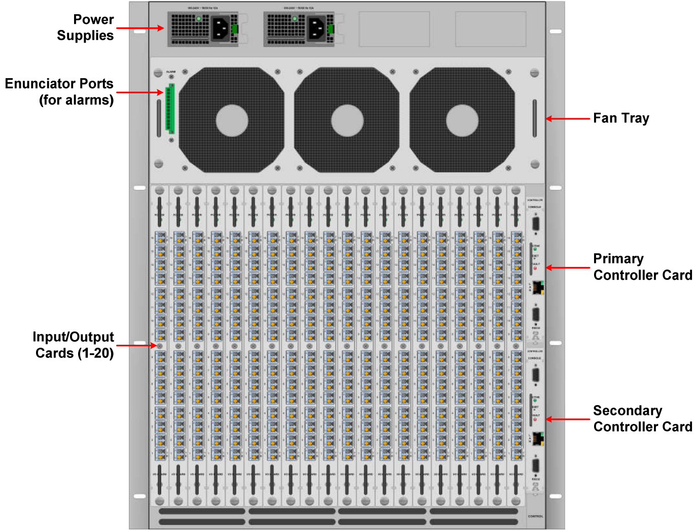
VX320VIDEO & VX320AUDIO Router – Rear View
