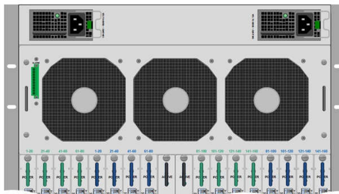
VX Router Power Supplies and Fan Tray with Alarm Annunciator
