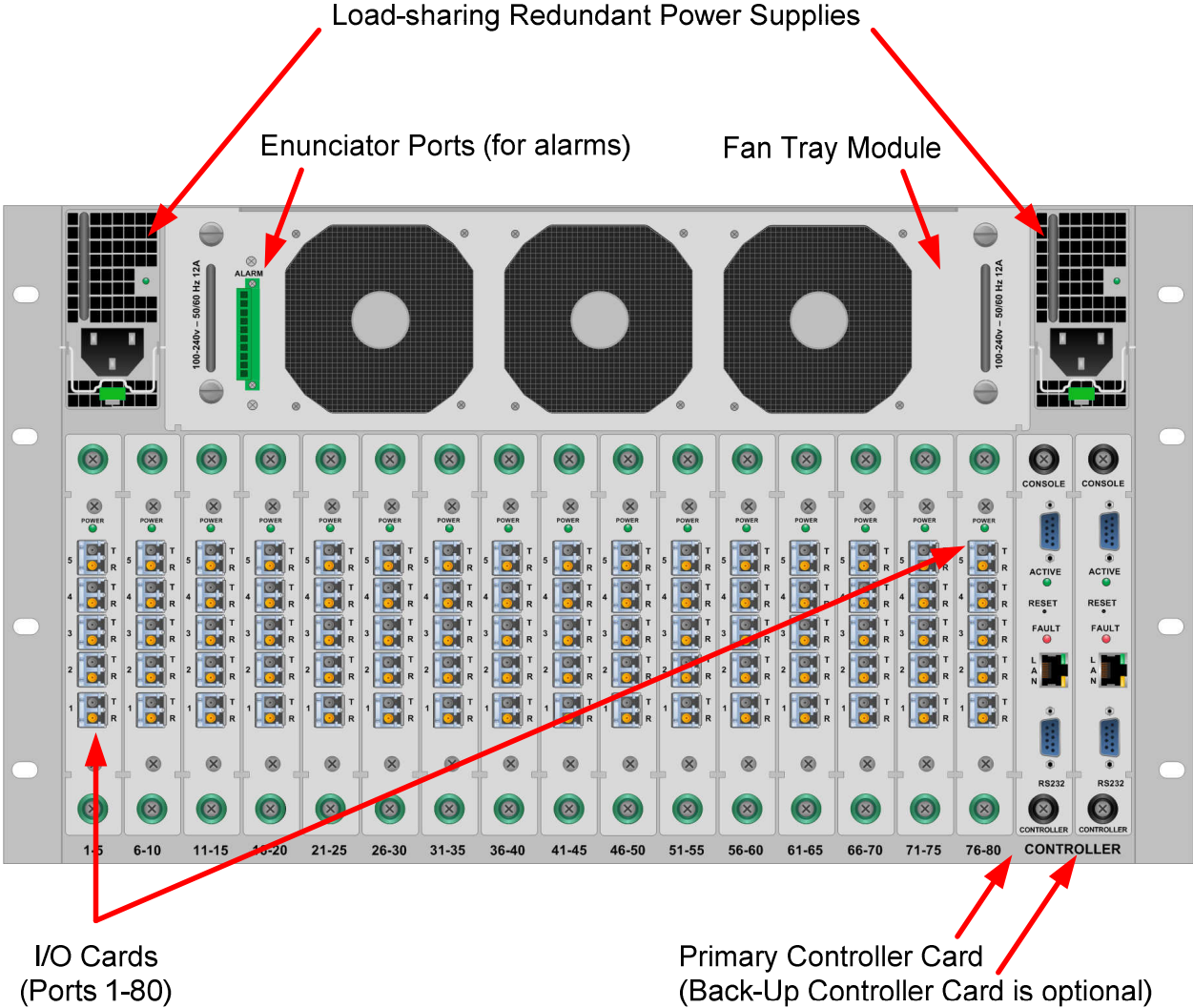
VX80 Router – Rear View
