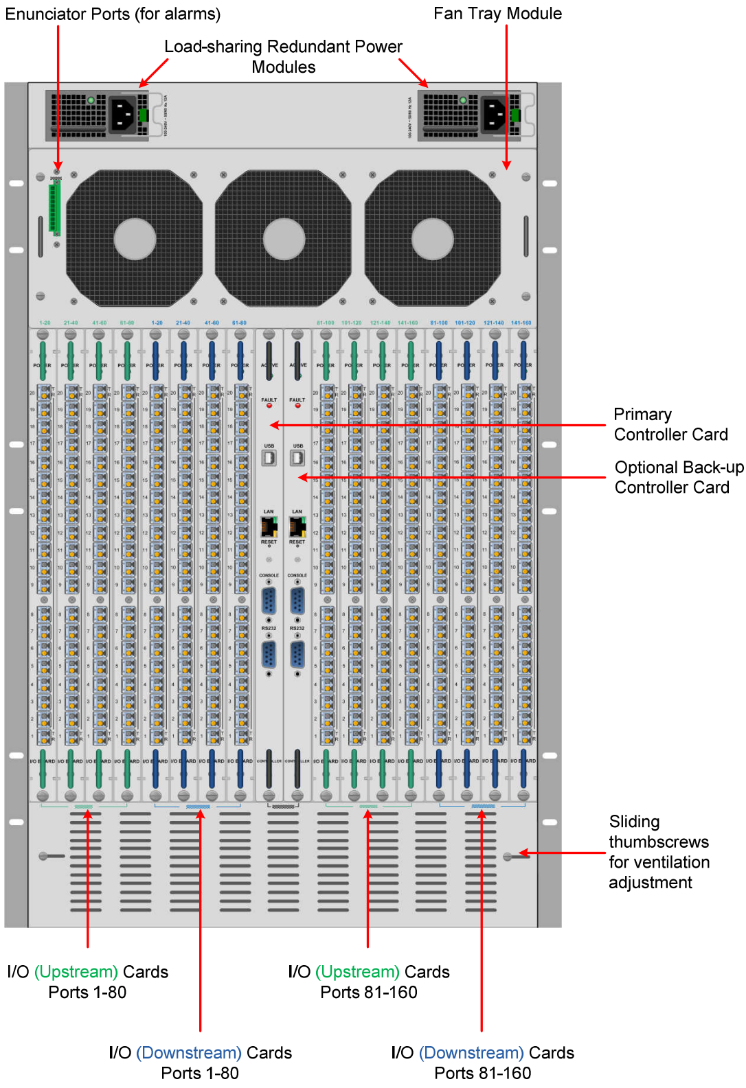
VX160 Router – Rear View
