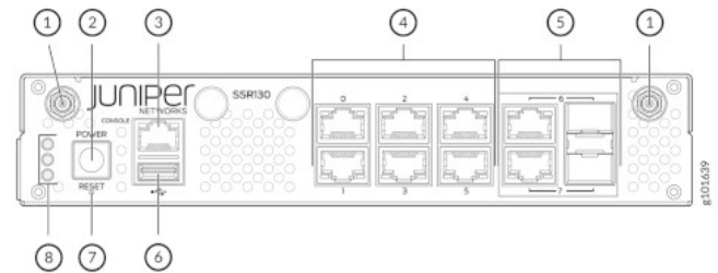
Figure 9. Front Panel Components of SSR130-AA and SSR130-AE
