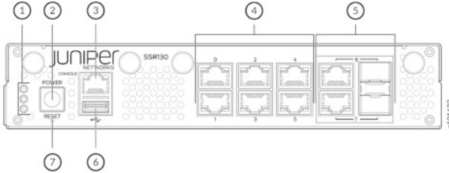
Figure 8. Front Panel Components of SSR130
