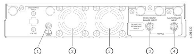
Figure 10. Rear Panel Components of an SSR130
