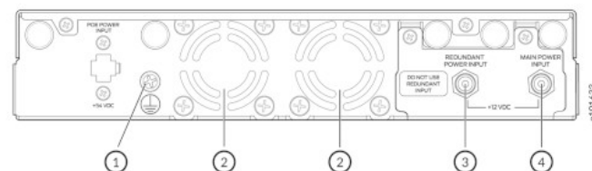
Figure 6. Rear Panel Components of SSR120
