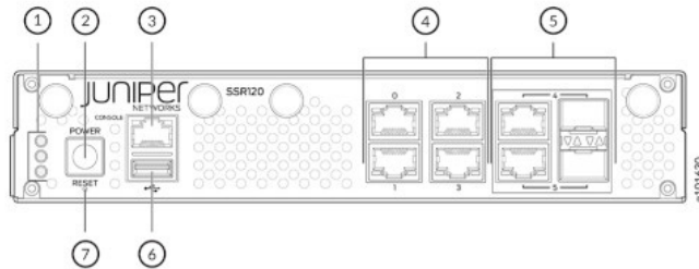
Figure 4. Front Panel Components of SSR120
