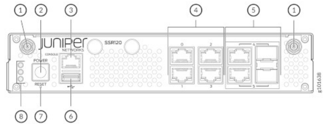
Figure 5. Front Panel Components of SSR120-AA and SSR120-AE
